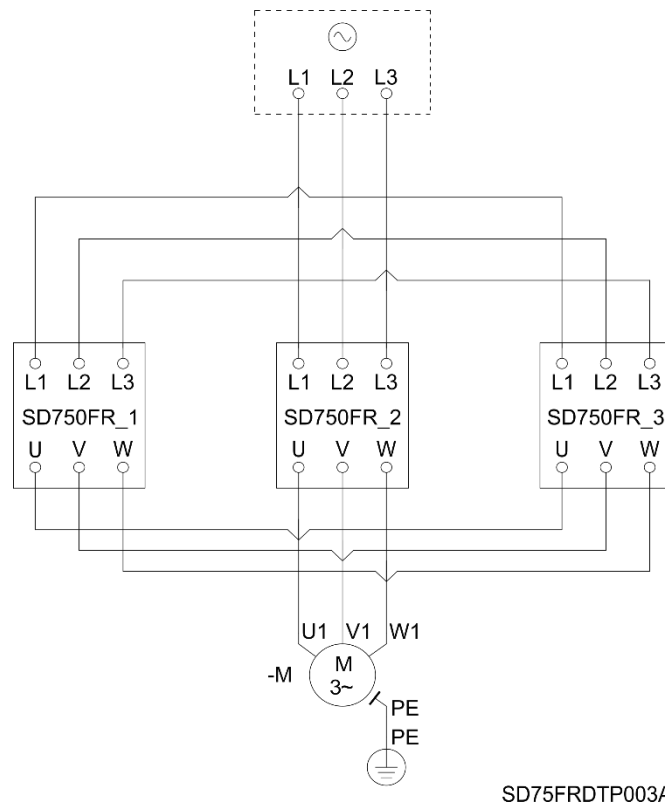
Power wiring connection for variable speed drives composed of three equipment of frame 9 to 11
