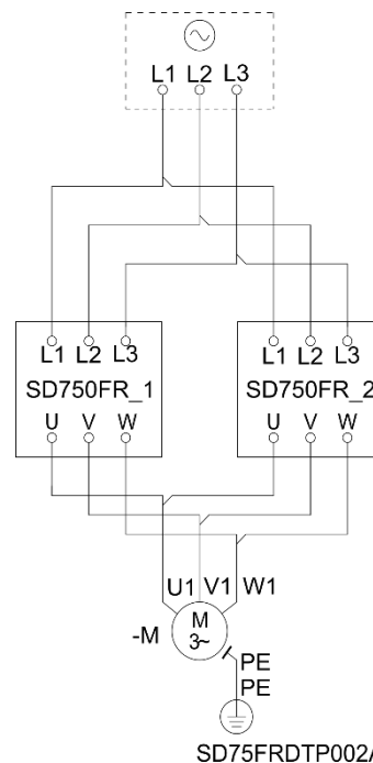
Power wiring connection for variable speed drives composed of two equipment of frame 9 to 11
